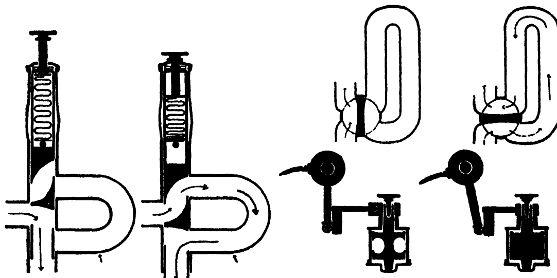
FIGURE 145. Piston and rotary valve, both in rest and action.
